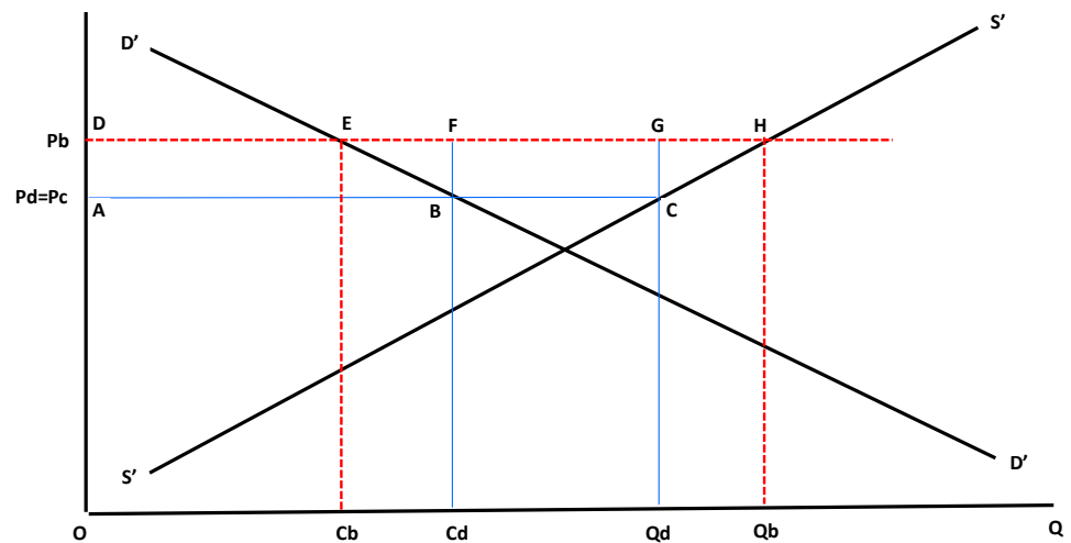
Figure 1. Partial equilibrium theory of trade (government price policy effects).
